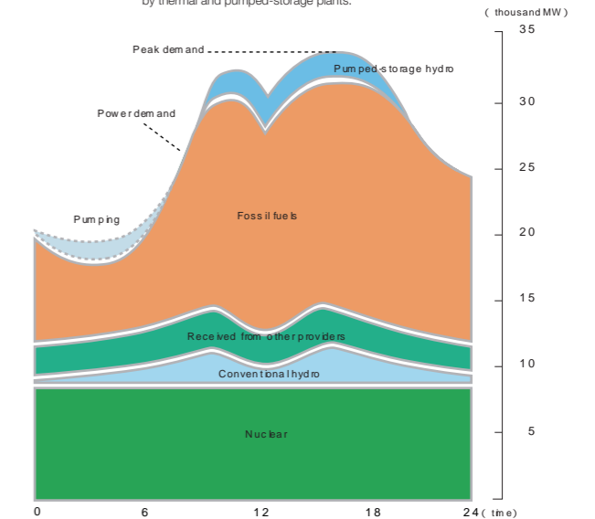
► 24-hour fluctuations in power demand and power sources (summer) ◀
